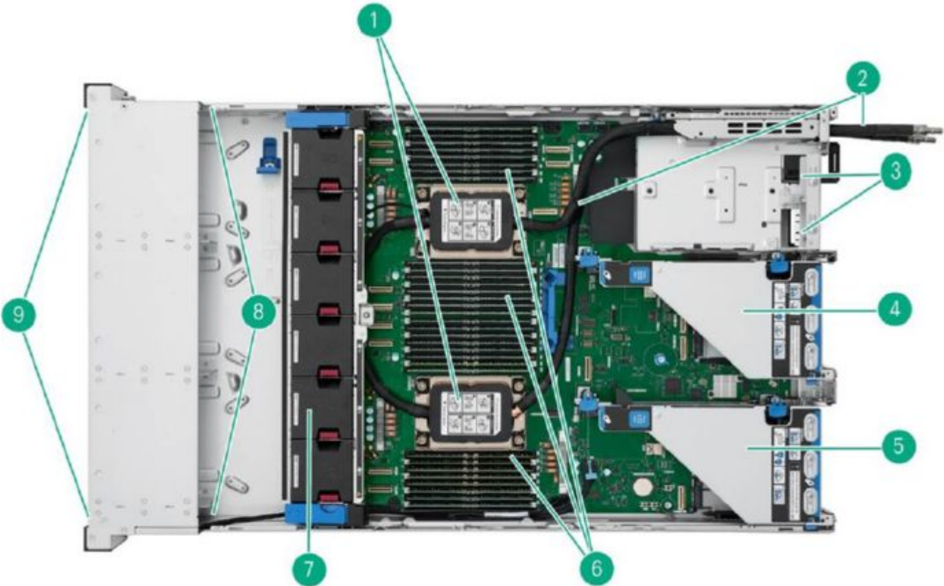
Internal View 12LFF Chassis - Direct Liquid Cooling
