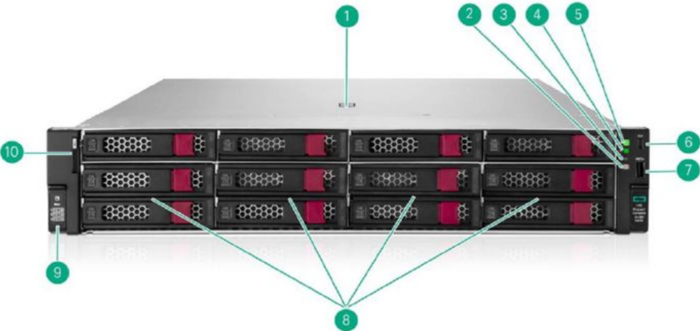
Front View - 12 LFF CTO Server
