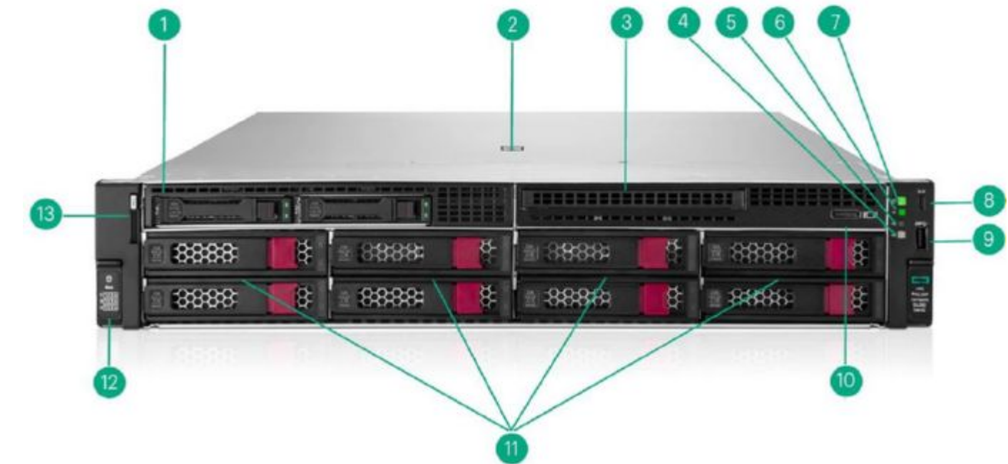
Front View - 8 LFF CTO Server with optional 2SFF and Universal Media Bay
