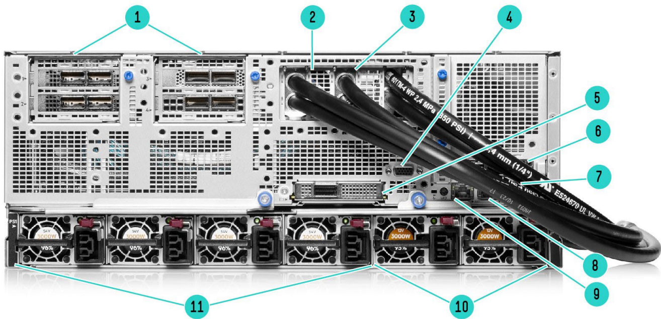
HPE Cray XD665 System Server Rear View
