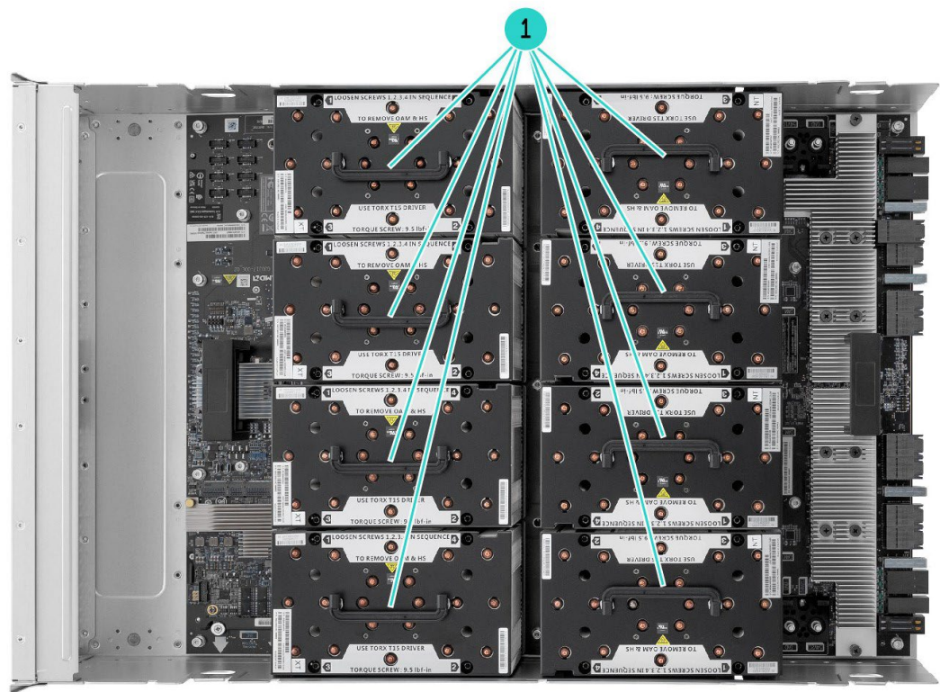
HPE Cray XD675 Server Top View
