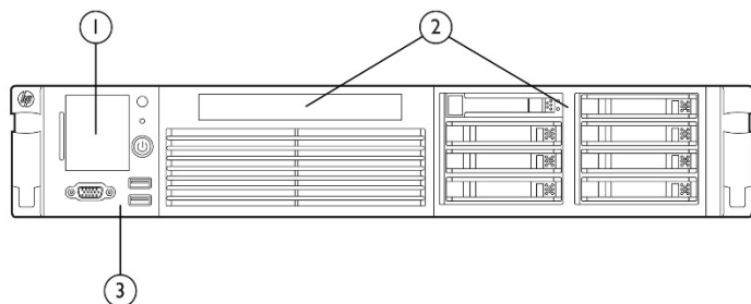
HPE Integrity rx2800 i6 Server: Front View
