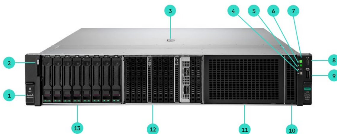
Front View – SFF chassis with optional EDSFF blank, OCP, and Drive Bay blank shown
