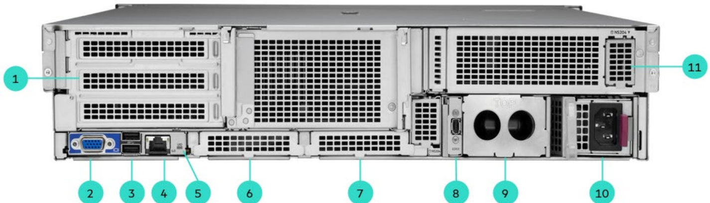
Rear View – SFF chassis
