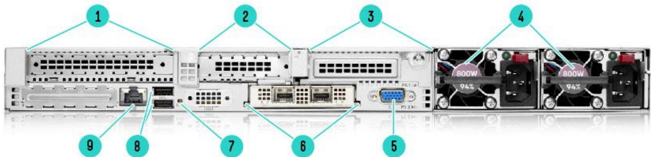
Rear View
