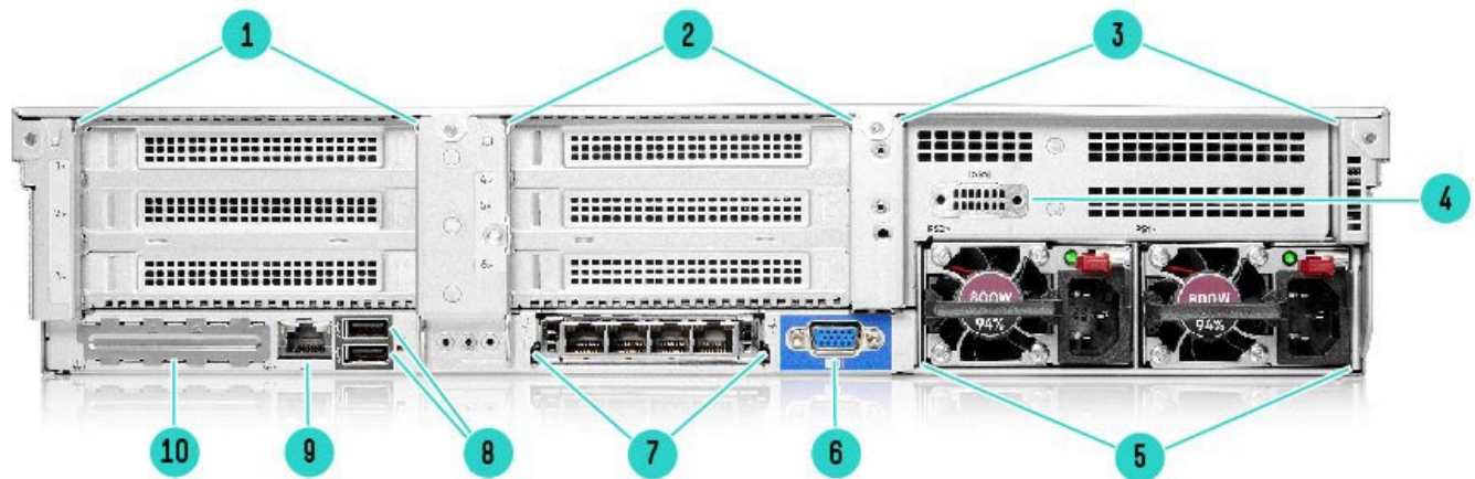
Rear View – Standard for all DX380 Gen10 Plus
