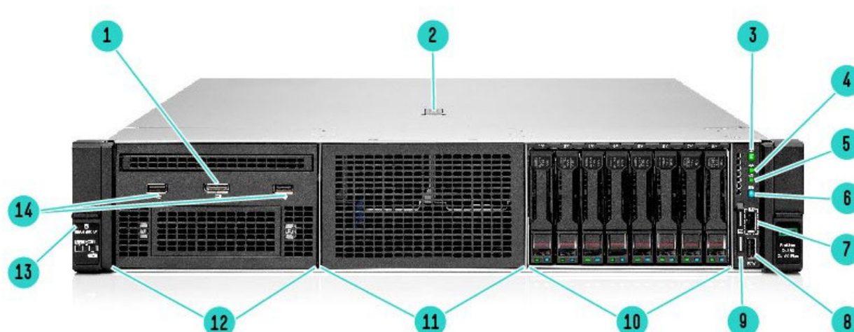
Front View – SFF chassis
